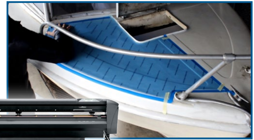
Prodim Procutter: Cuts templates from foil
